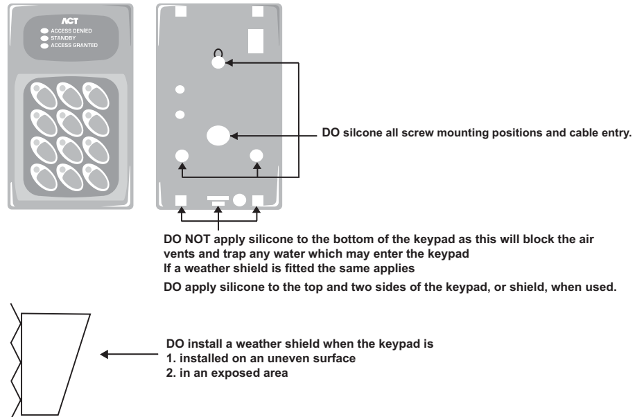
Figure 3: ACT 10 Digital Keypad - Guide to outdoor installation in exposed areas
