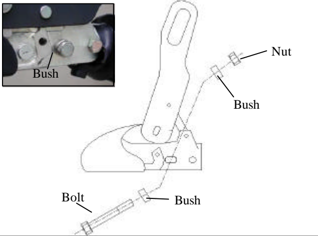
Illustration of front horizontal bolt.
